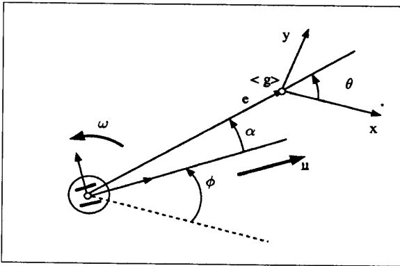
Figure 1. Vehicle's position and orientation with respect to the target frame.
