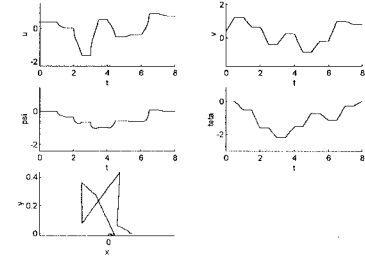
Figure 5: Path from \mathbf{x}_0 = [0, 0, \frac{\pi}{8}, \frac{\pi}{8}, 0, 0] to \mathbf{x}_1 = [0, 0, \frac{\pi}{4}, -\frac{\pi}{4}, 0, 0] .
