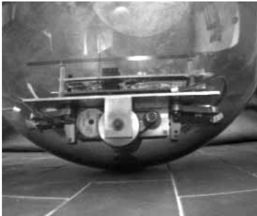
Figure 1: The prototype in our laboratory
