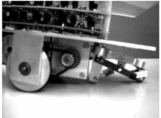
Figure 2: A close-up of the inner vehicle showing the stepper motors and the suspension system
