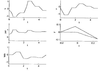
Figure 4: Path from \mathbf{x}_0 = [0, 0, -\frac{\pi}{8}, -\frac{\pi}{8}, \frac{\pi}{8}, 0] to \mathbf{x}_1 = [0, 0, -\frac{\pi}{8}, -\frac{\pi}{8}, \frac{\pi}{4}, 0] . The plot in x - y coordinates describes the path followed by the vehicle in the plane.
