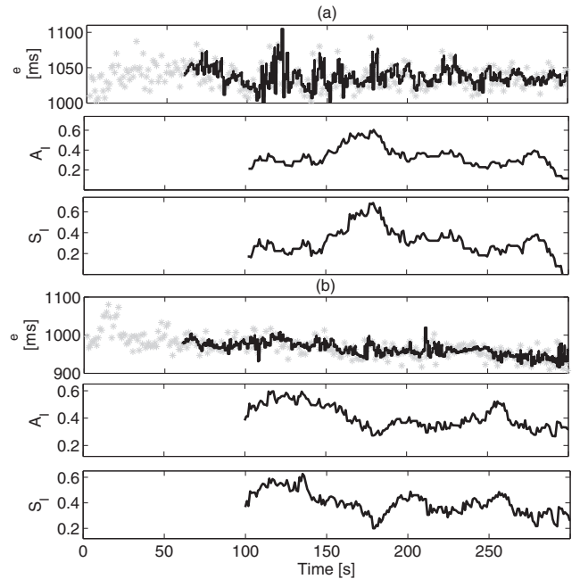
FIG. 7. Instantaneous statistics computed from a representative healthy (a) and elderly (b) subject of the gait dynamics dataset, computed using a NARL model. From the top, given the interevent interval e (gray asterisks), the estimated \mu_e(t) (continuous line), superimposed on the recorded e series is shown. Below, the instantaneous A_I and S_I complexity tracking are shown.
